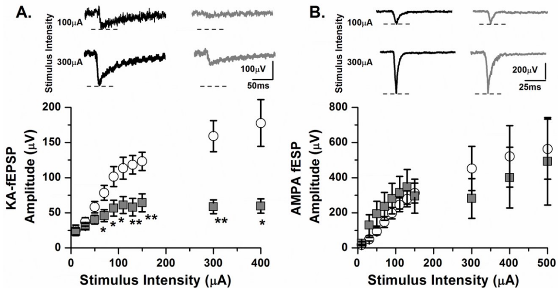
Figure 5.7. I/O curves of mossy fiber evoked fEPSPs demonstrate a selective decrease in KAR-mediated transmission. A. The amplitude of the fEPSP KA evoked from pilo-treated animals (closed gray squares, n = 4 - 6 ) is significantly reduced compared to the fEPSP KA evoked from sham-treated animals (open circles, n = 3 - 6 ) at stimulus intensities of 70 – 400 \mu\text{A} . Representative waveforms from sham-treated (black traces) and pilo-treated (gray traces) demonstrate the reduced potentiation of fEPSP KA at two different stimulus intensities. B. The amplitude of the fEPSP AMPA evoked from pilo-treated animals (closed gray squares, n = 3 - 5 ) is not significantly different than the fEPSP AMPA evoked from sham-treated animals (open circles, n = 4 - 10 ) at any of the stimulus intensities examined. Representative waveforms from sham-treated (black traces) and pilo-treated (gray traces) are not different at two different stimulus intensities. * p < 0.05 ; ** p < 0.01 , t-test.
